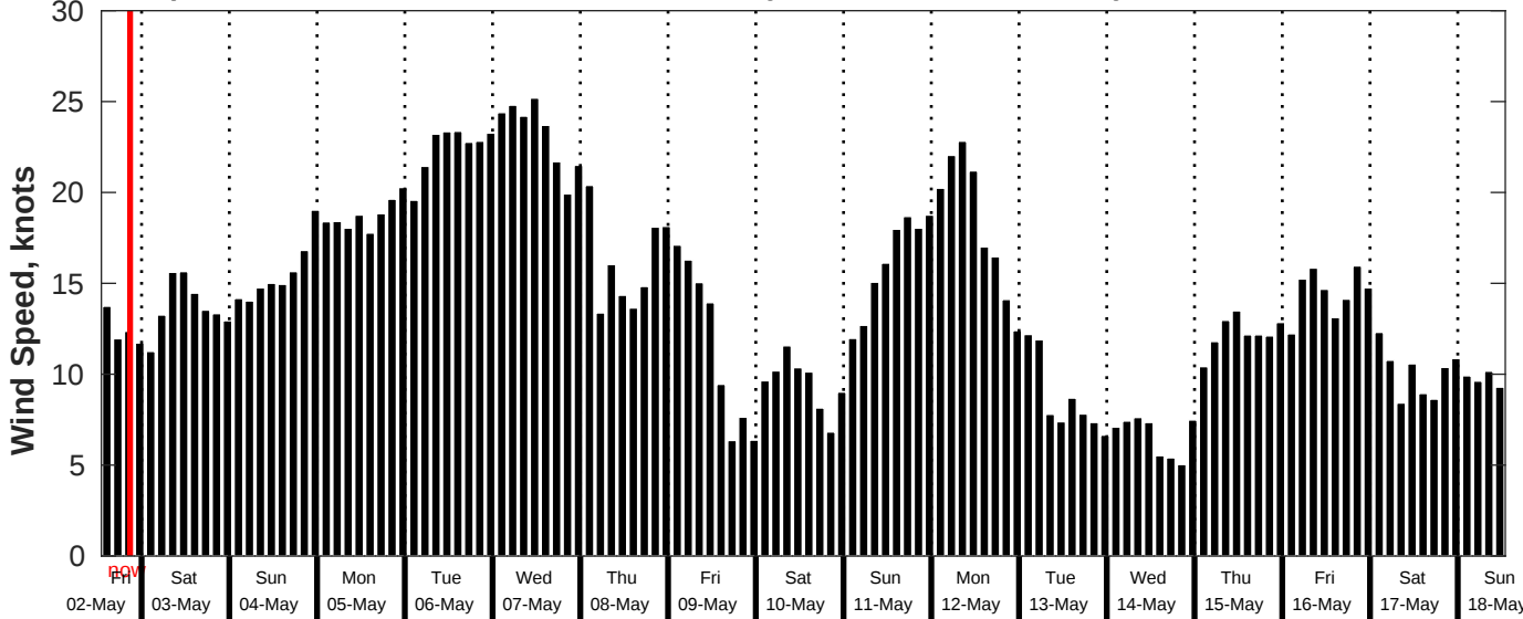
GFS Wind Speed Forecast for NDBC 51209 from 02-May-2025 13:00:00 to 18-May-2025 13:00:00
