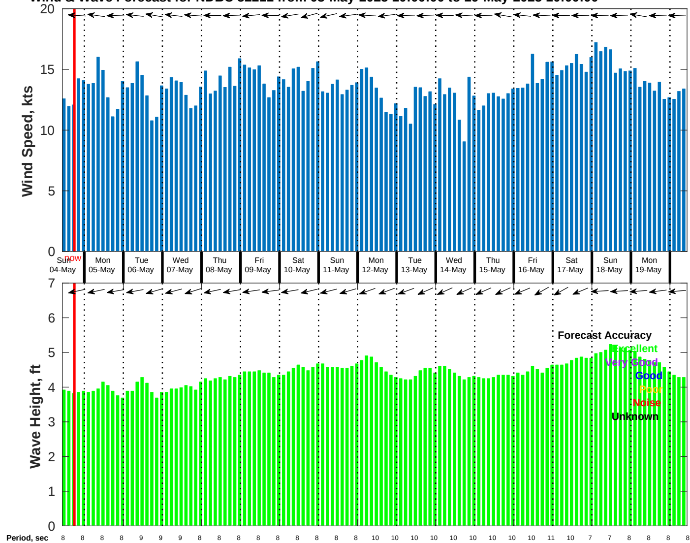
Wind & Wave Forecast for NDBC 52211 from 03-May-2025 10:00:00 to 19-May-2025 10:00:00
