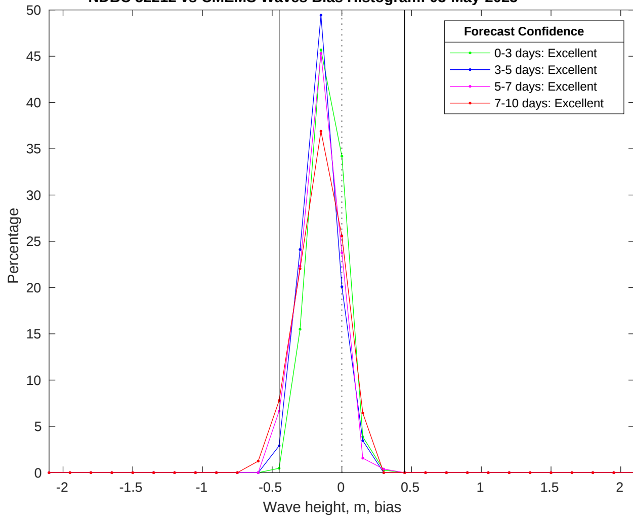
NDBC 52212 vs CMEMS Waves Bias Histogram: 03-May-2025
