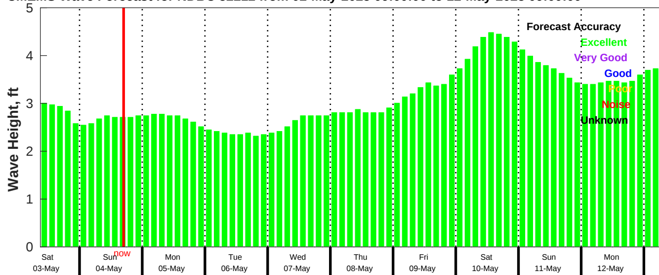
CMEMS Wave Forecast for NDBC 52212 from 02-May-2025 09:00:00 to 12-May-2025 09:00:00
