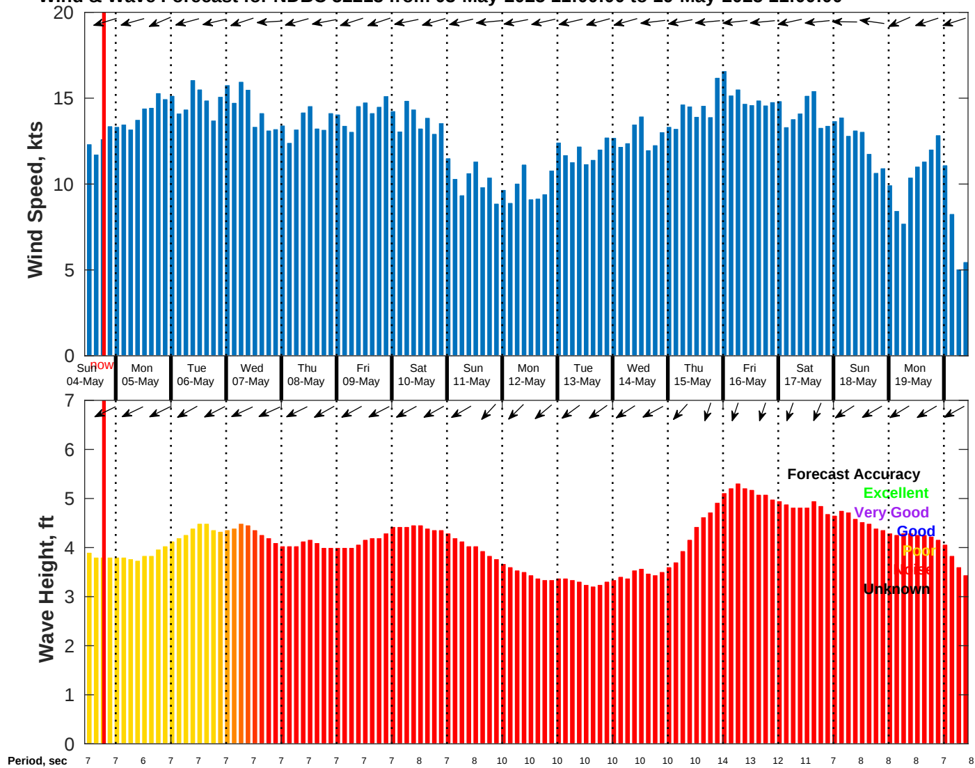
Wind & Wave Forecast for NDBC 52213 from 03-May-2025 11:00:00 to 19-May-2025 11:00:00
