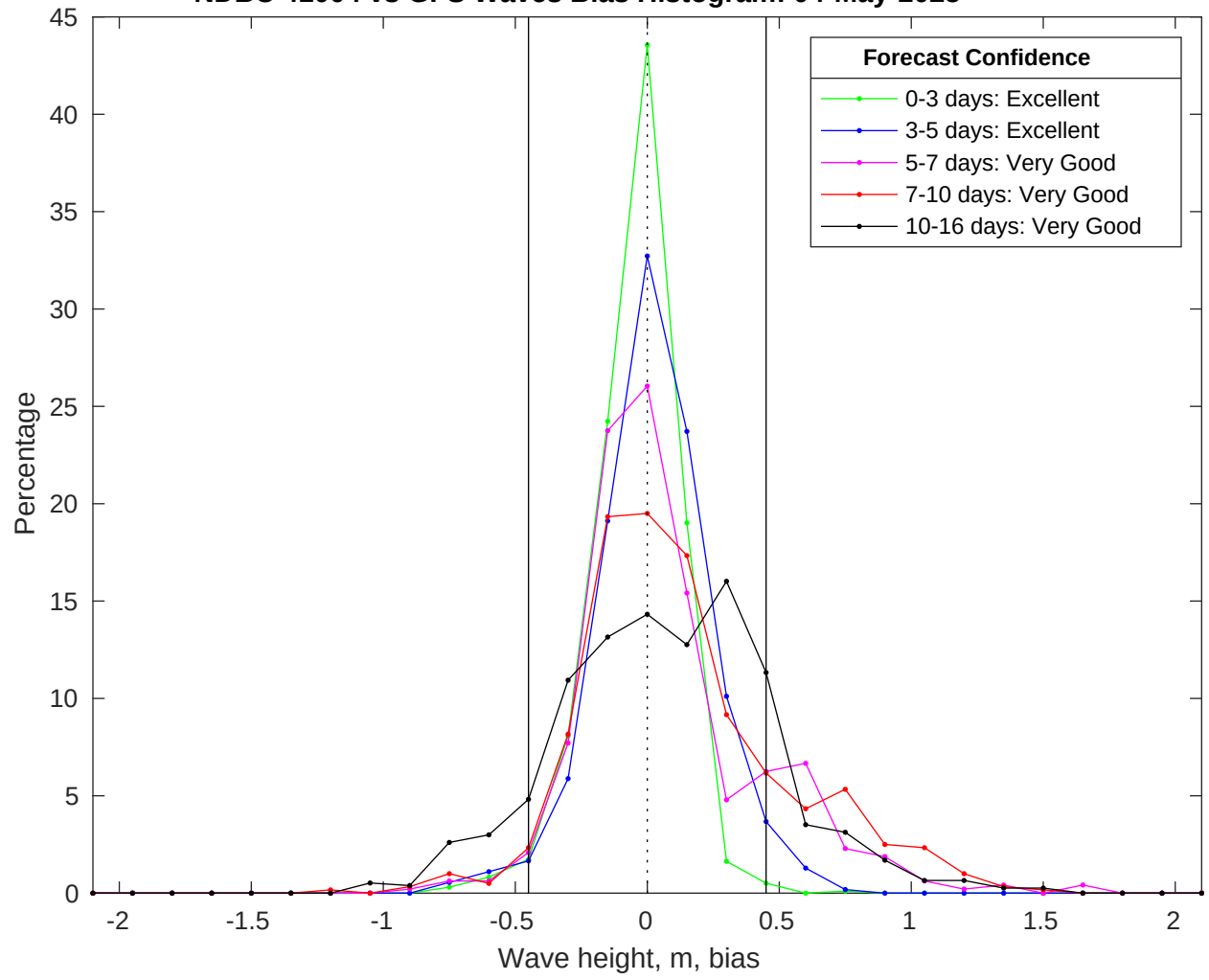
NDBC 41004 vs GFS Waves Bias Histogram: 04-May-2025
