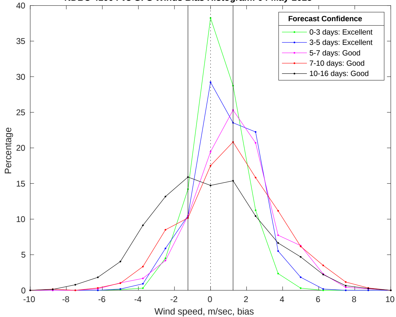
NDBC 41004 vs GFS Winds Bias Histogram: 04-May-2025
