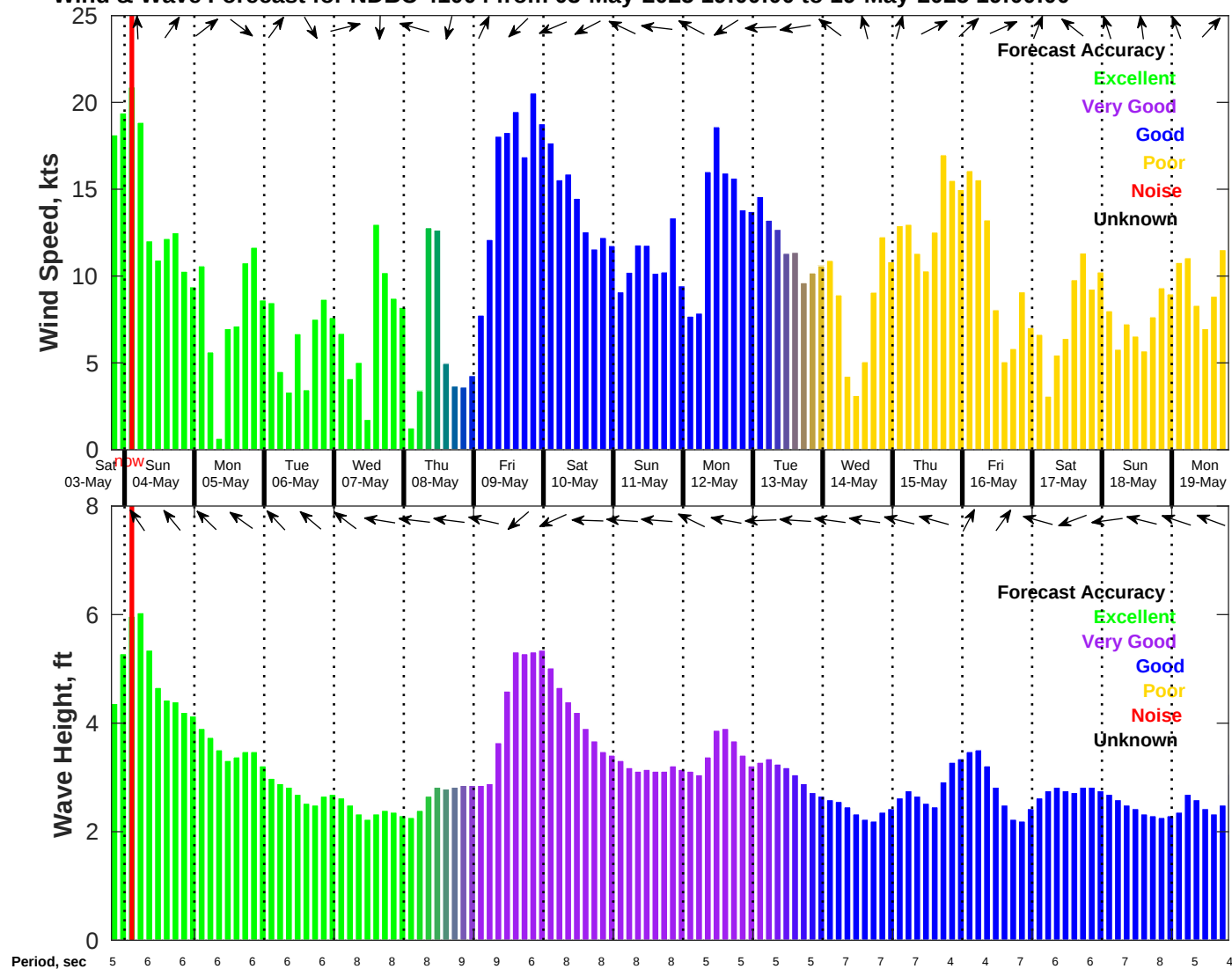
Wind & Wave Forecast for NDBC 41004 from 03-May-2025 19:00:00 to 19-May-2025 19:00:00
