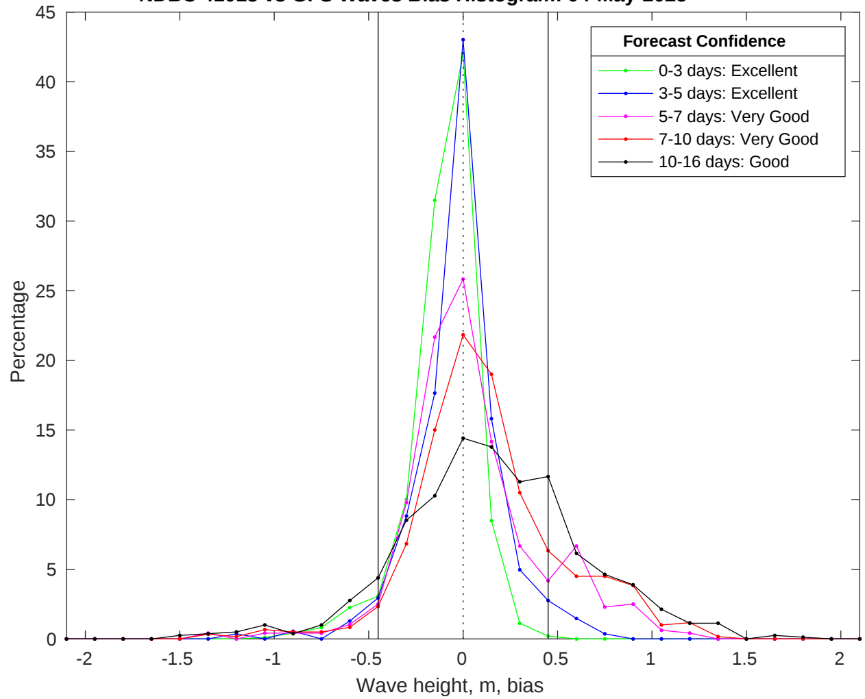
NDBC 41013 vs GFS Waves Bias Histogram: 04-May-2025
