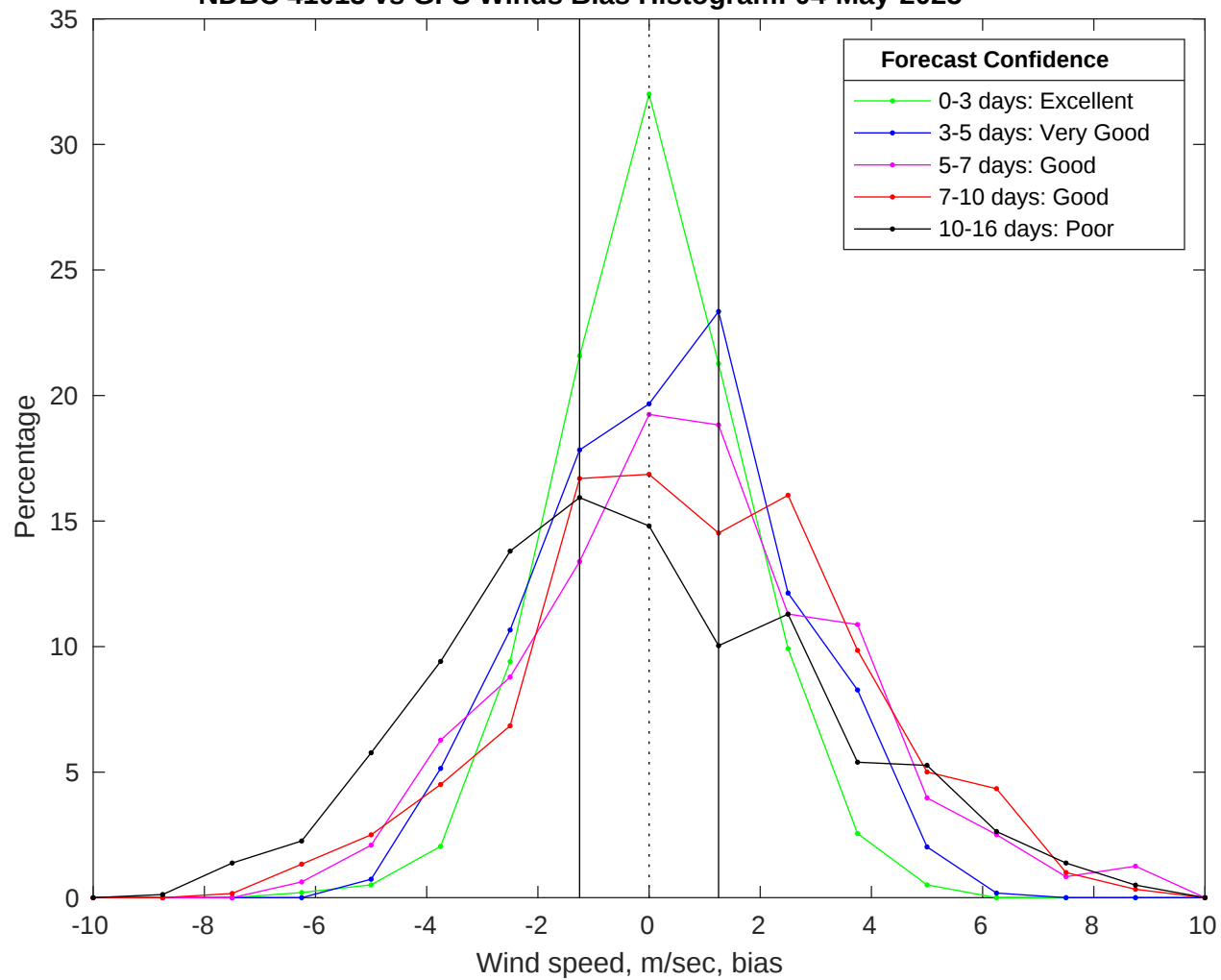
NDBC 41013 vs GFS Winds Bias Histogram: 04-May-2025
