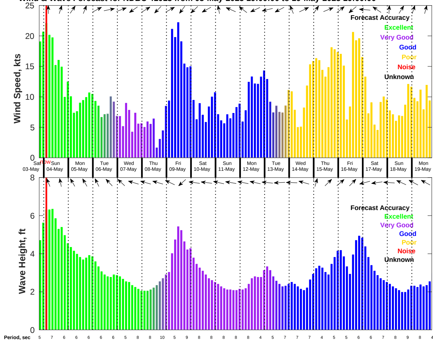
Wind & Wave Forecast for NDBC 41013 from 03-May-2025 19:00:00 to 19-May-2025 19:00:00
