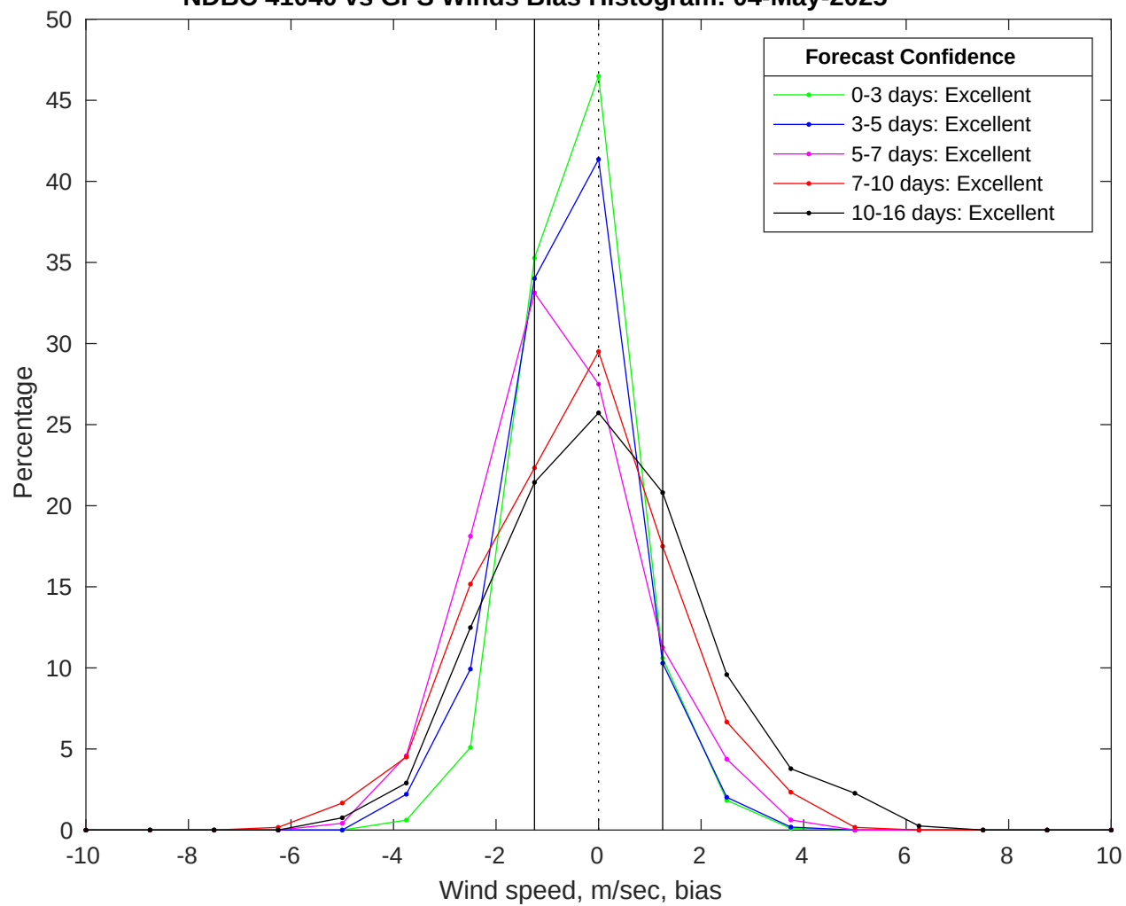
NDBC 41040 vs GFS Winds Bias Histogram: 04-May-2025
