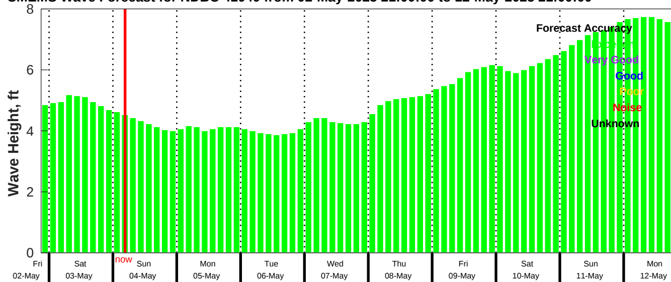
CMEMS Wave Forecast for NDBC 41040 from 02-May-2025 21:00:00 to 12-May-2025 21:00:00
