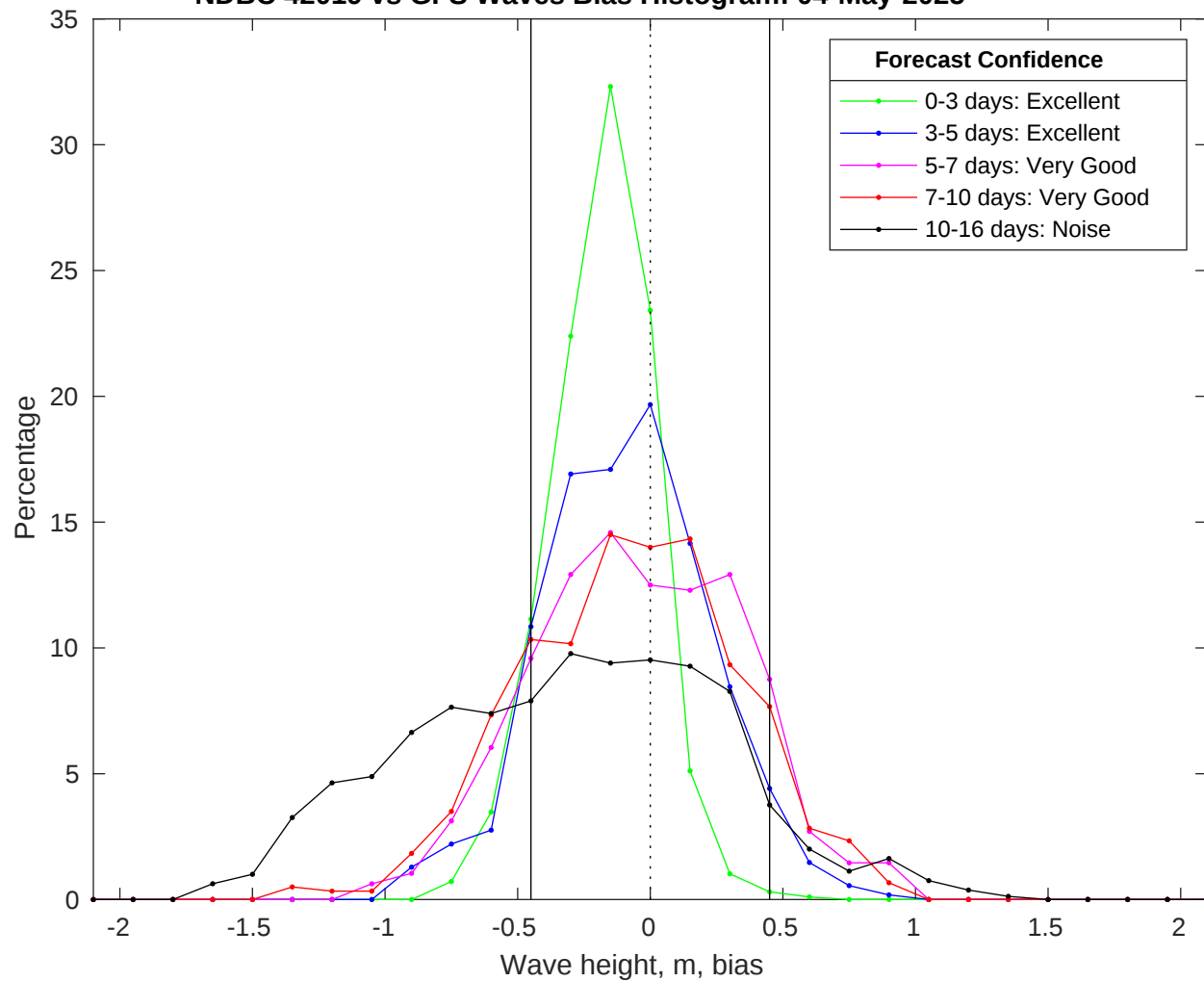
NDBC 42019 vs GFS Waves Bias Histogram: 04-May-2025
