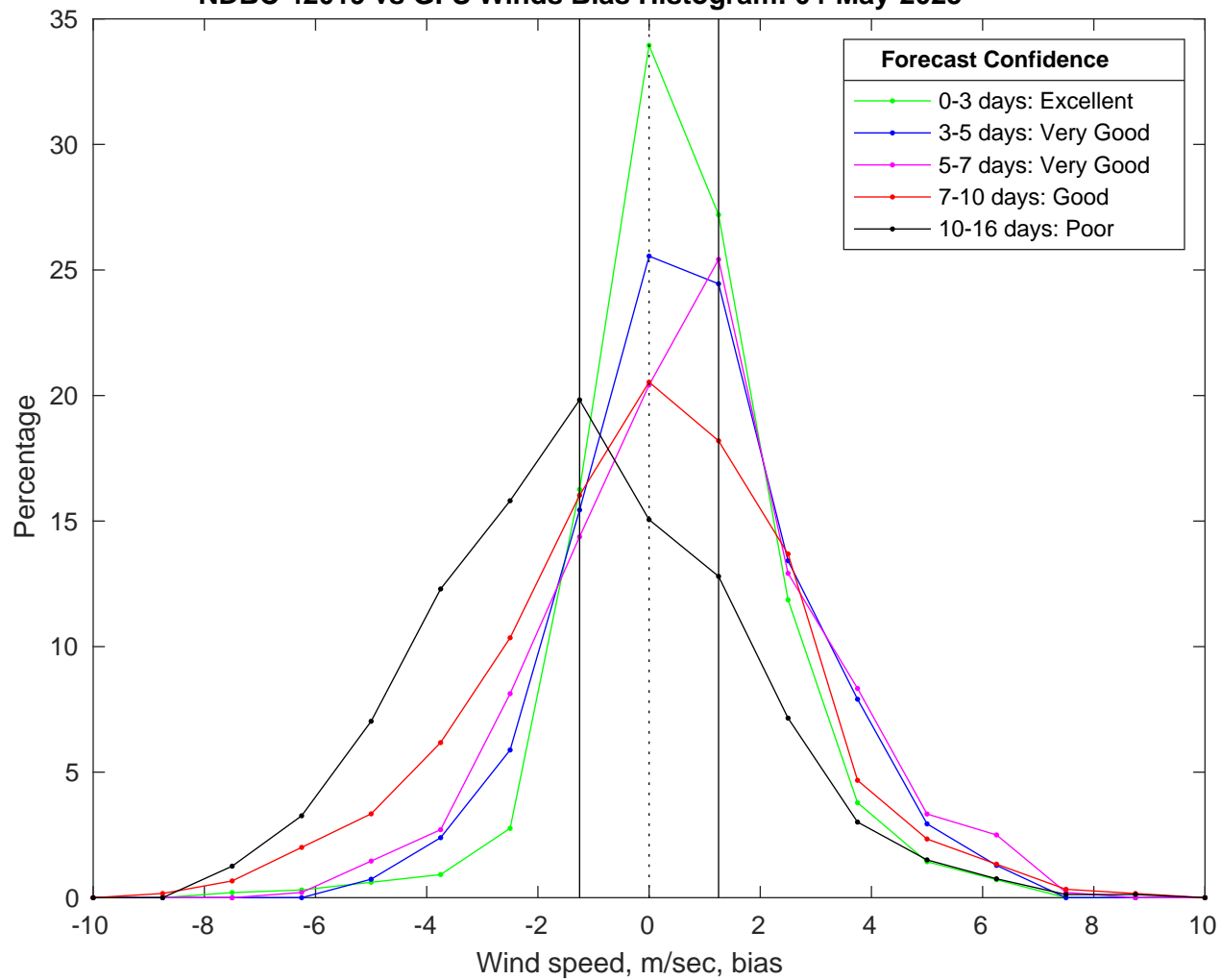
NDBC 42019 vs GFS Winds Bias Histogram: 04-May-2025
