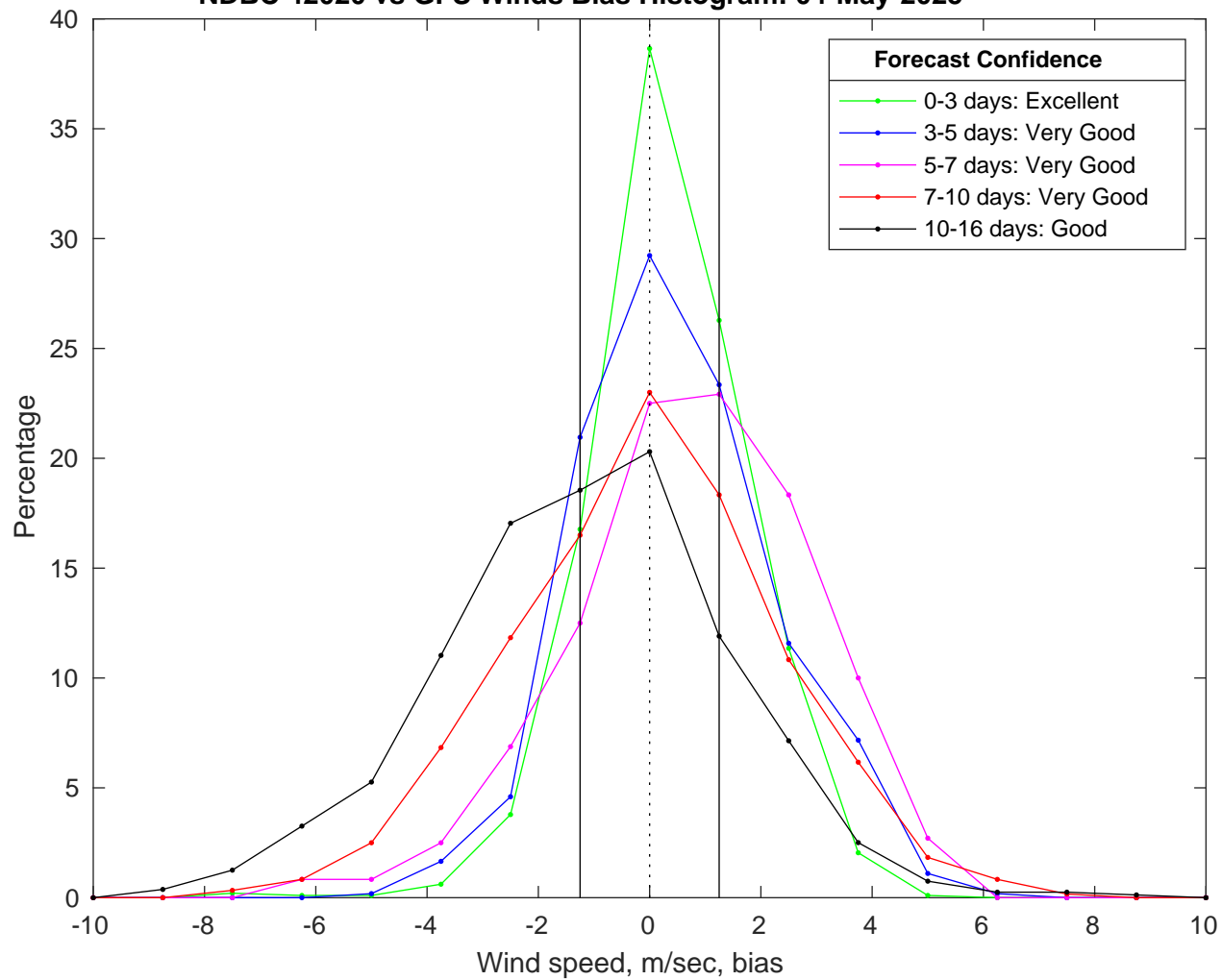
NDBC 42020 vs GFS Winds Bias Histogram: 04-May-2025
