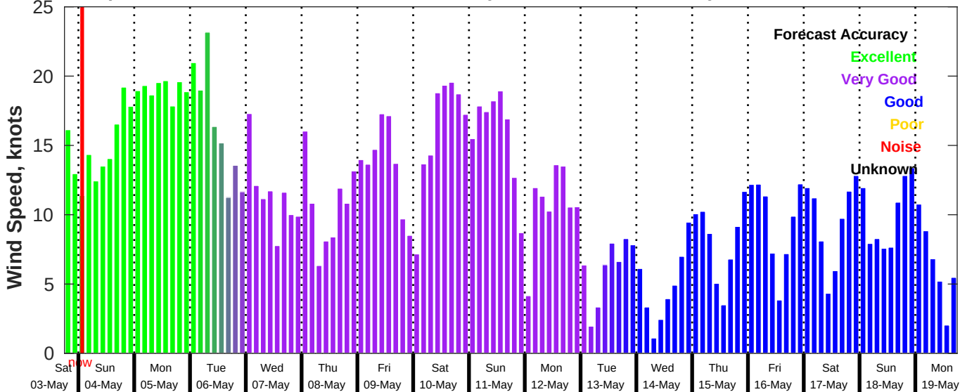
GFS Wind Speed Forecast for NDBC 42020 from 03-May-2025 18:00:00 to 19-May-2025 18:00:00
