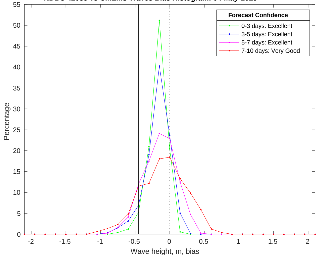
NDBC 42035 vs CMEMS Waves Bias Histogram: 04-May-2025
