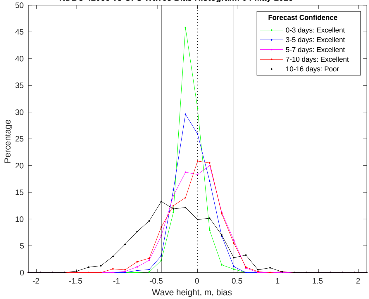
NDBC 42035 vs GFS Waves Bias Histogram: 04-May-2025
