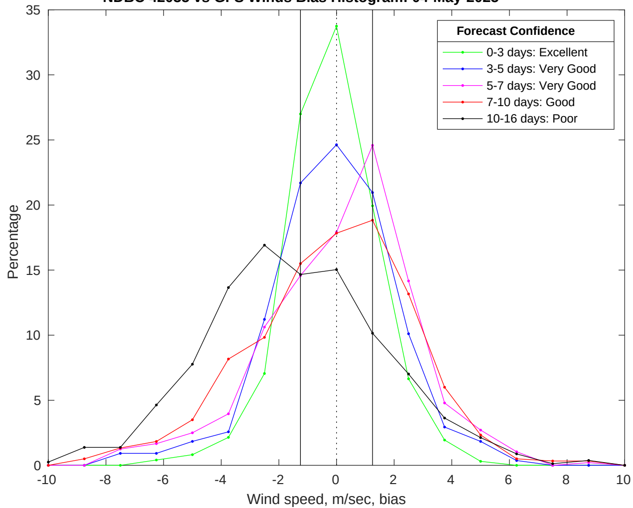
NDBC 42035 vs GFS Winds Bias Histogram: 04-May-2025
