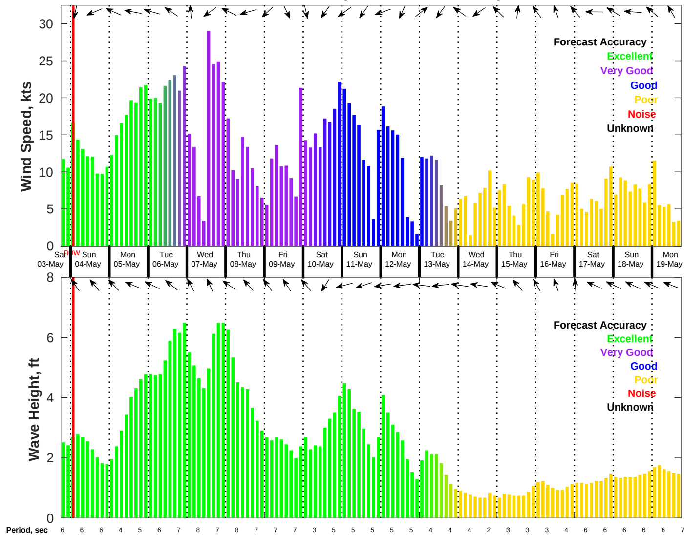
Wind & Wave Forecast for NDBC 42035 from 03-May-2025 18:00:00 to 19-May-2025 18:00:00
