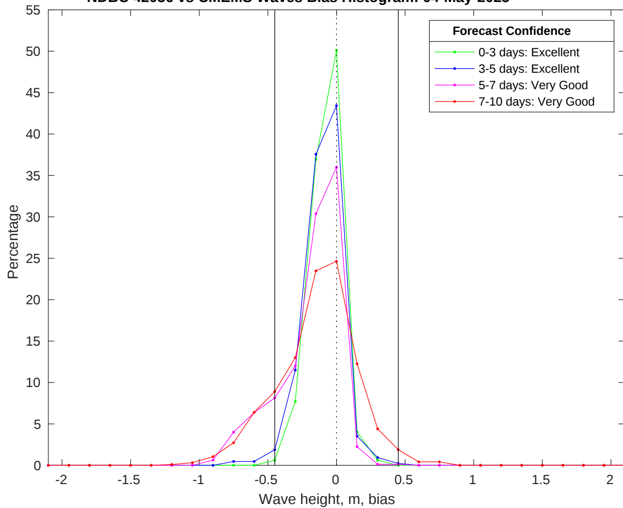
NDBC 42036 vs CMEMS Waves Bias Histogram: 04-May-2025
