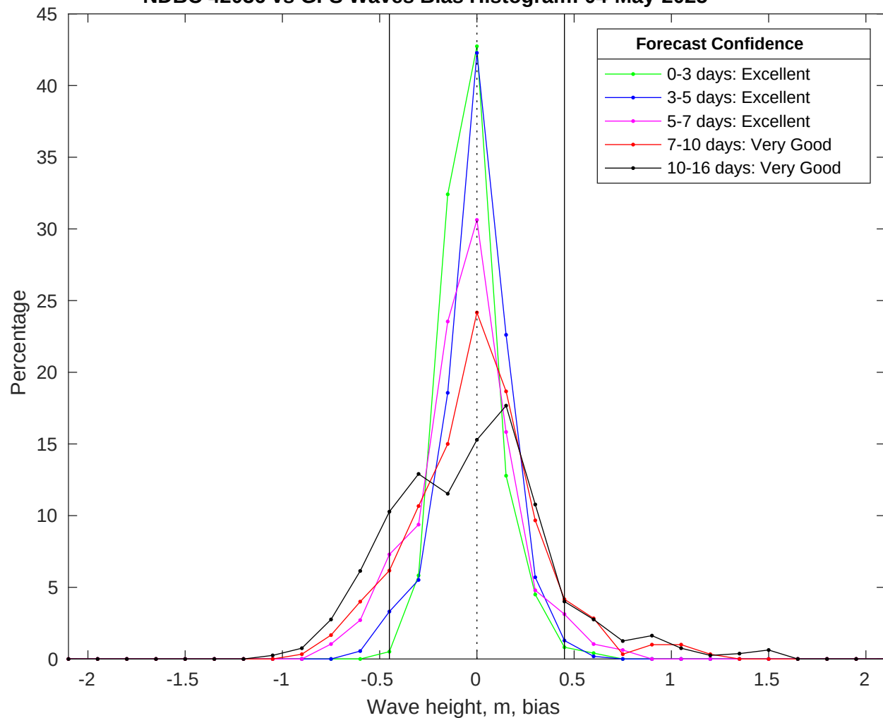
NDBC 42036 vs GFS Waves Bias Histogram: 04-May-2025
