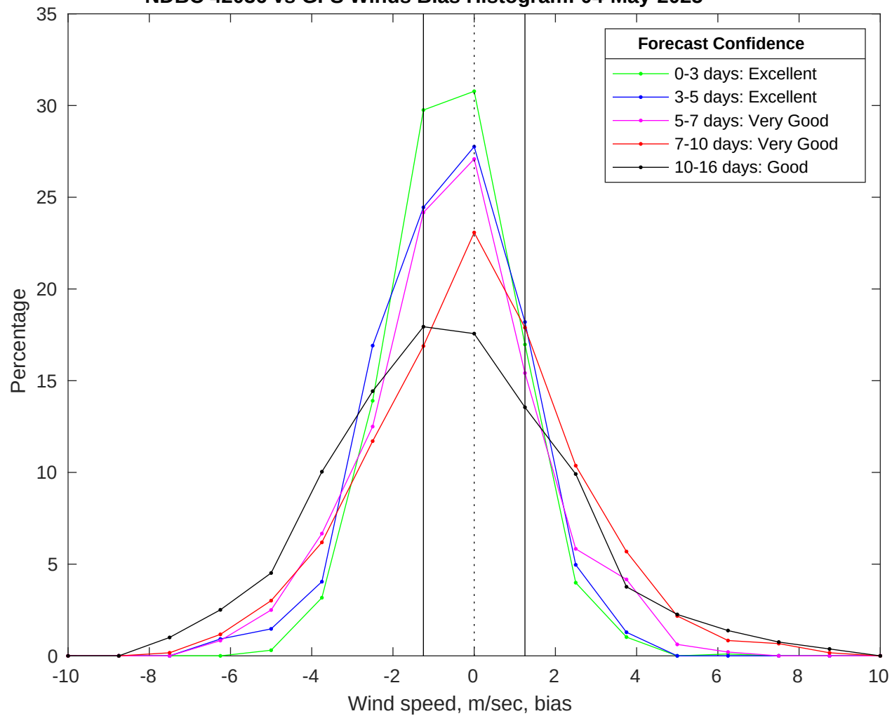
NDBC 42036 vs GFS Winds Bias Histogram: 04-May-2025
