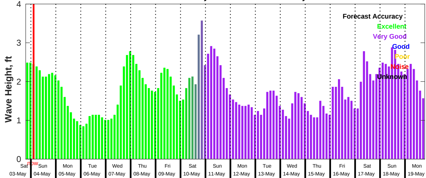
GFS Wave Forecast for NDBC 42036 from 03-May-2025 19:00:00 to 19-May-2025 19:00:00
