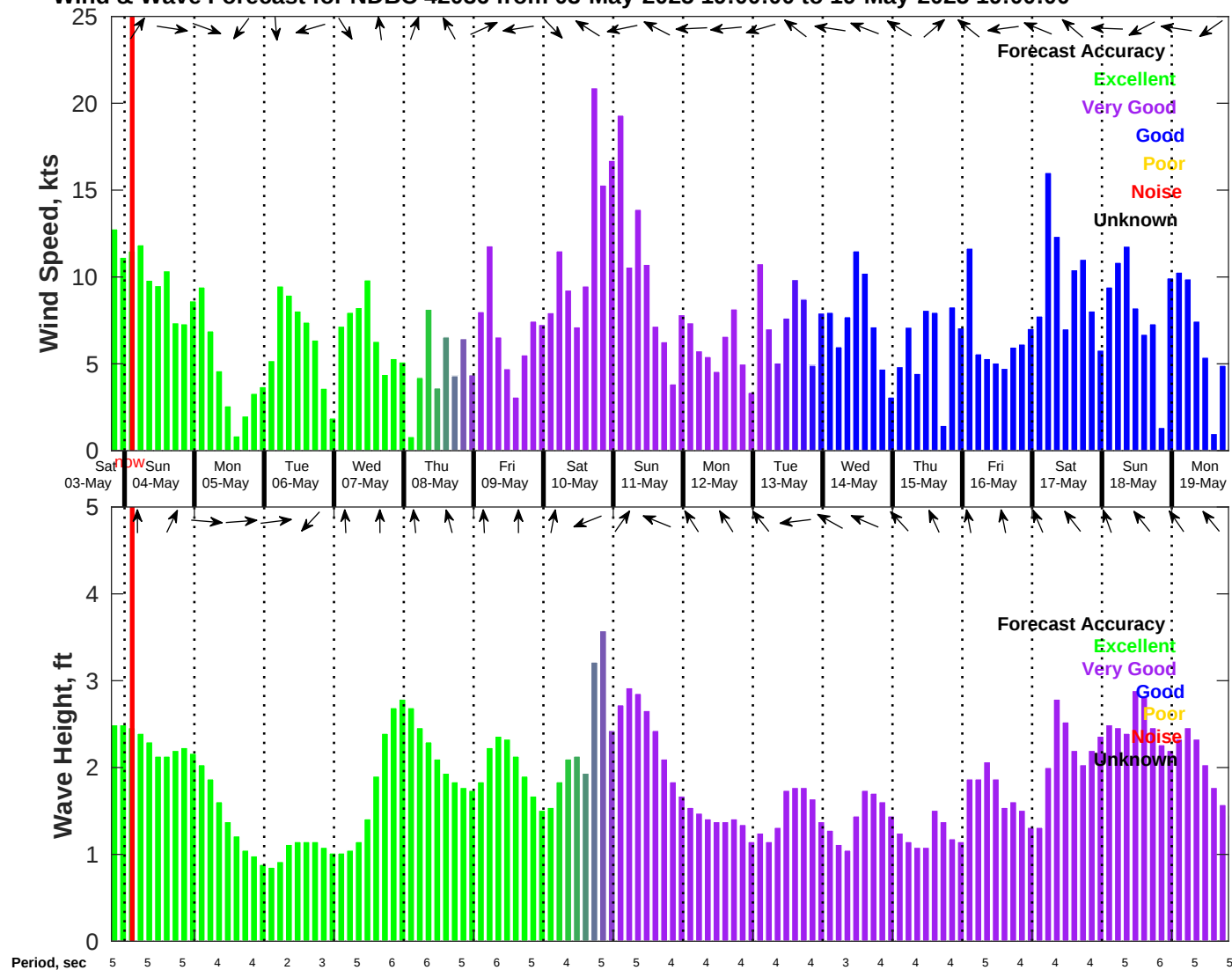
Wind & Wave Forecast for NDBC 42036 from 03-May-2025 19:00:00 to 19-May-2025 19:00:00
