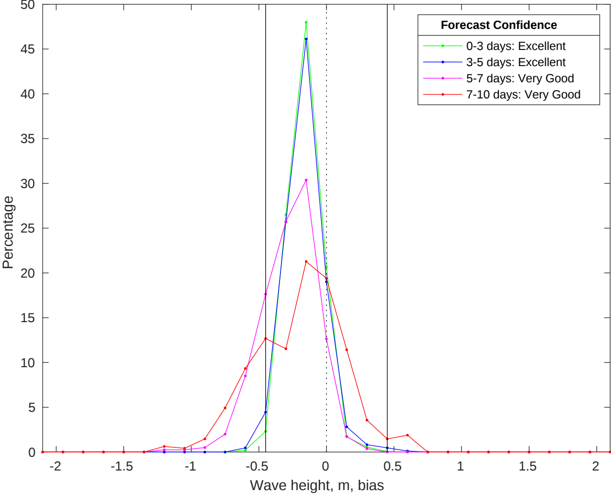
NDBC 42040 vs CMEMS Waves Bias Histogram: 04-May-2025
