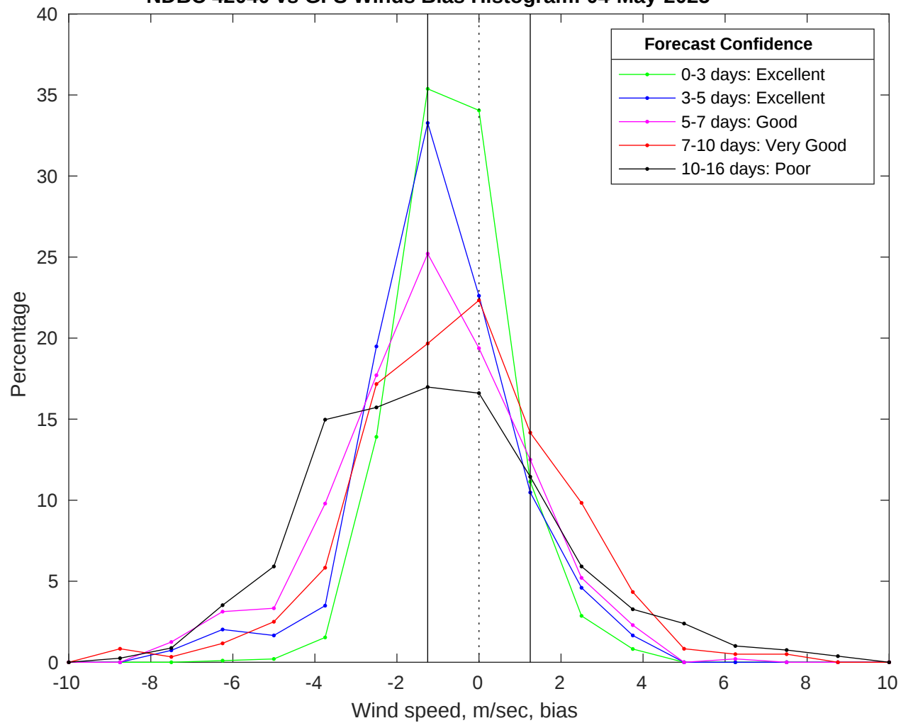
NDBC 42040 vs GFS Winds Bias Histogram: 04-May-2025
