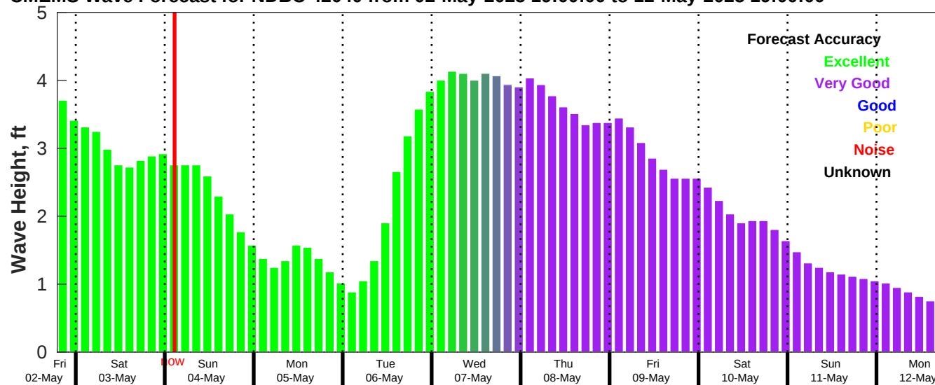
CMEMS Wave Forecast for NDBC 42040 from 02-May-2025 19:00:00 to 12-May-2025 19:00:00
