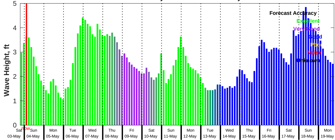
GFS Wave Forecast for NDBC 42040 from 03-May-2025 19:00:00 to 19-May-2025 19:00:00
