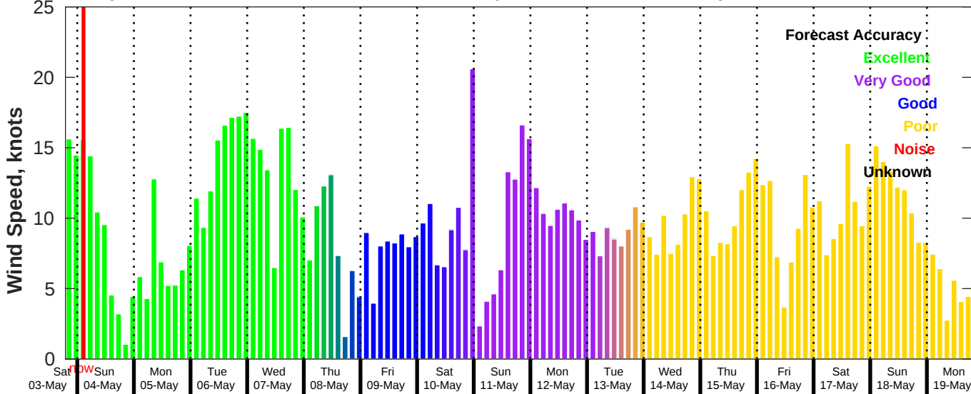
GFS Wind Speed Forecast for NDBC 42040 from 03-May-2025 19:00:00 to 19-May-2025 19:00:00
