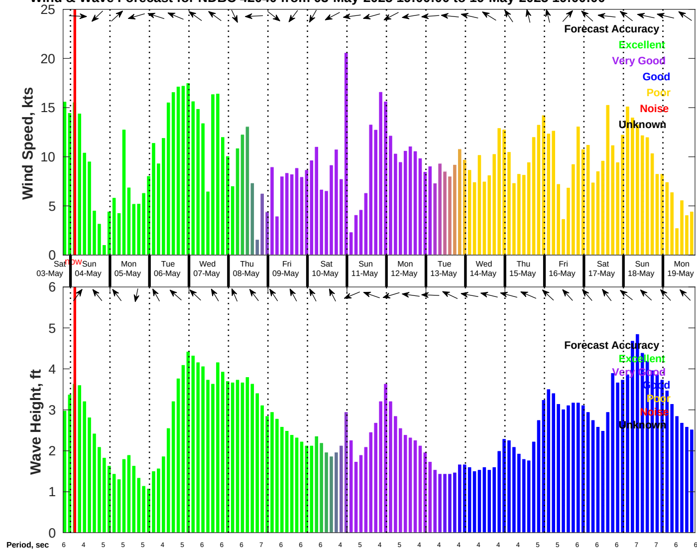
Wind & Wave Forecast for NDBC 42040 from 03-May-2025 19:00:00 to 19-May-2025 19:00:00
