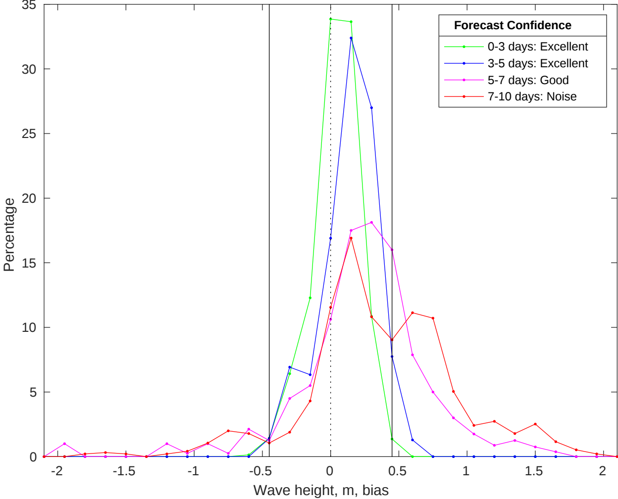
NDBC 46011 vs CMEMS Waves Bias Histogram: 04-May-2025
