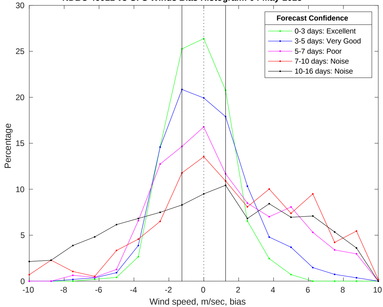
NDBC 46011 vs GFS Winds Bias Histogram: 04-May-2025
