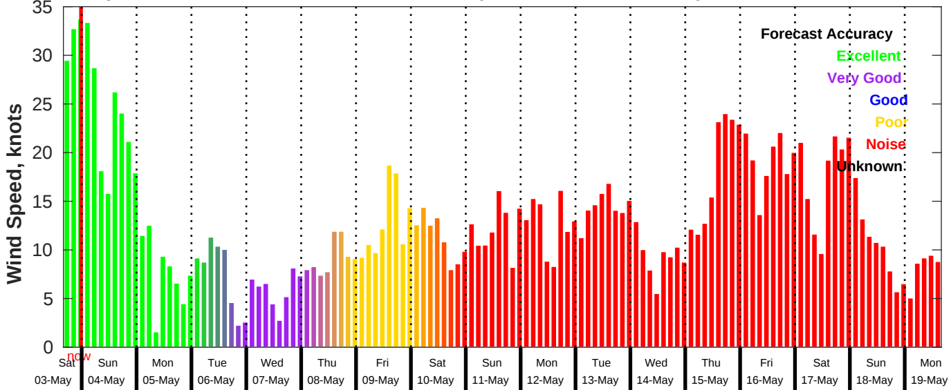
GFS Wind Speed Forecast for NDBC 46011 from 03-May-2025 16:00:00 to 19-May-2025 16:00:00
