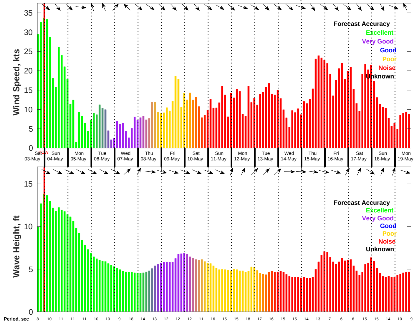
Wind & Wave Forecast for NDBC 46011 from 03-May-2025 16:00:00 to 19-May-2025 16:00:00
