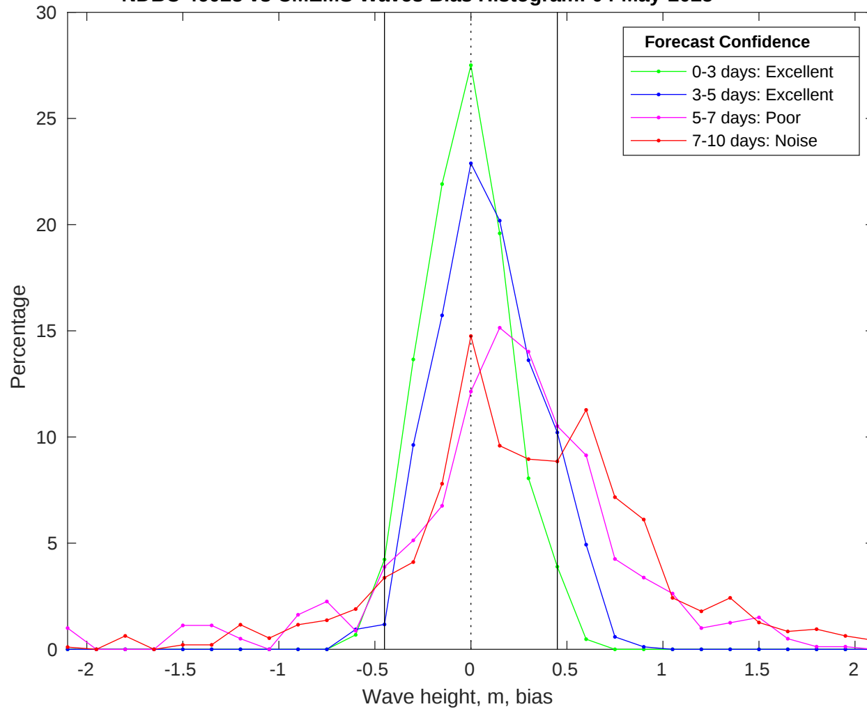
NDBC 46028 vs CMEMS Waves Bias Histogram: 04-May-2025
