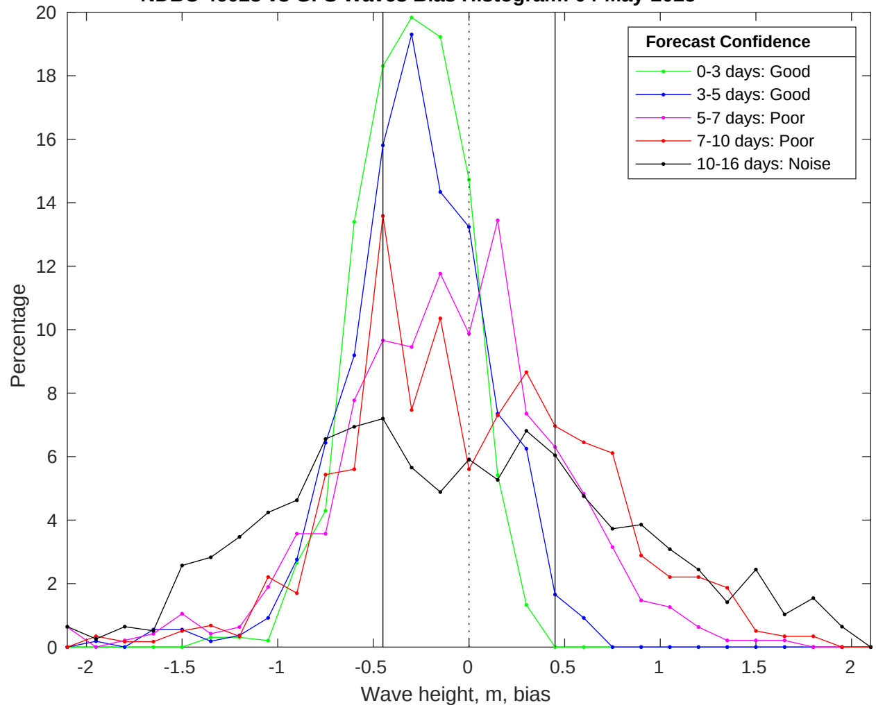
NDBC 46028 vs GFS Waves Bias Histogram: 04-May-2025
