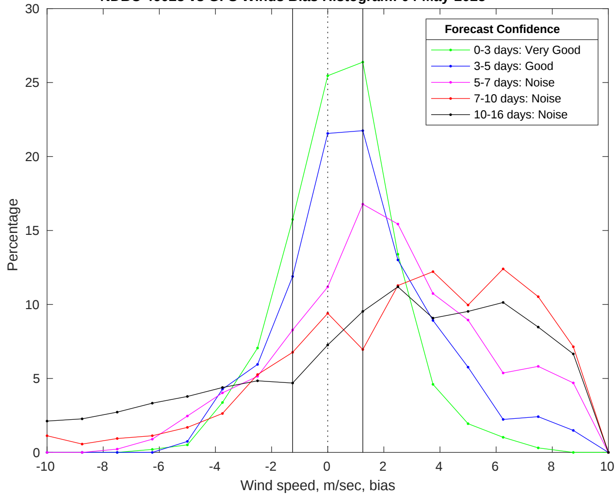
NDBC 46028 vs GFS Winds Bias Histogram: 04-May-2025
