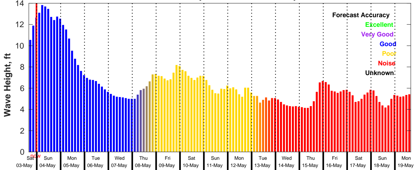
GFS Wave Forecast for NDBC 46028 from 03-May-2025 16:00:00 to 19-May-2025 16:00:00
