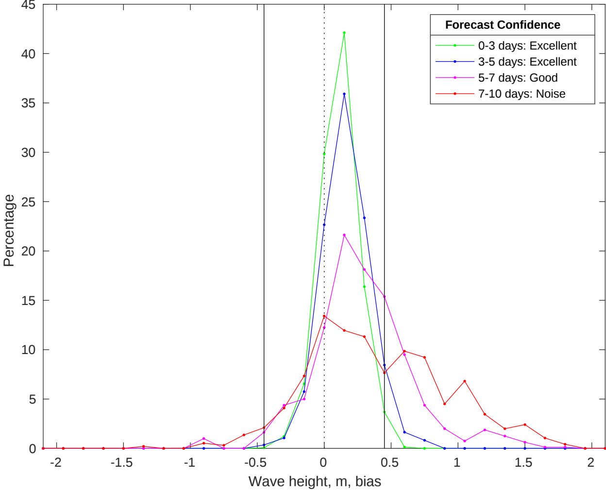
NDBC 46054 vs CMEMS Waves Bias Histogram: 04-May-2025
