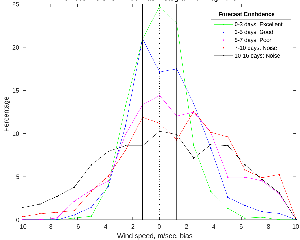
NDBC 46054 vs GFS Winds Bias Histogram: 04-May-2025
