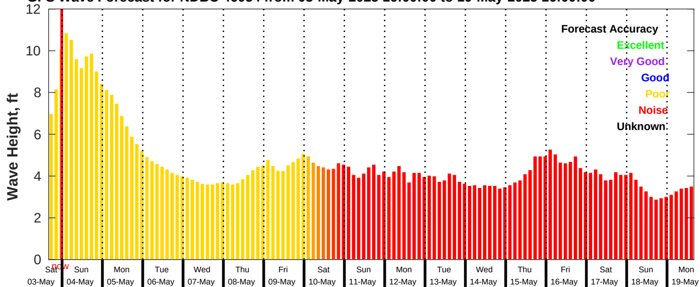
GFS Wave Forecast for NDBC 46054 from 03-May-2025 16:00:00 to 19-May-2025 16:00:00
