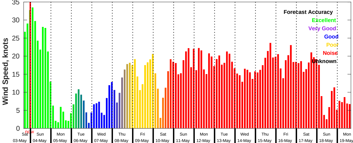
GFS Wind Speed Forecast for NDBC 46054 from 03-May-2025 16:00:00 to 19-May-2025 16:00:00
