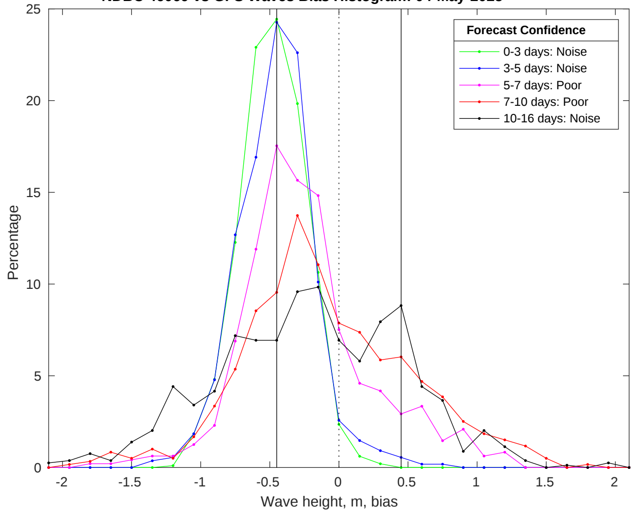
NDBC 46069 vs GFS Waves Bias Histogram: 04-May-2025
