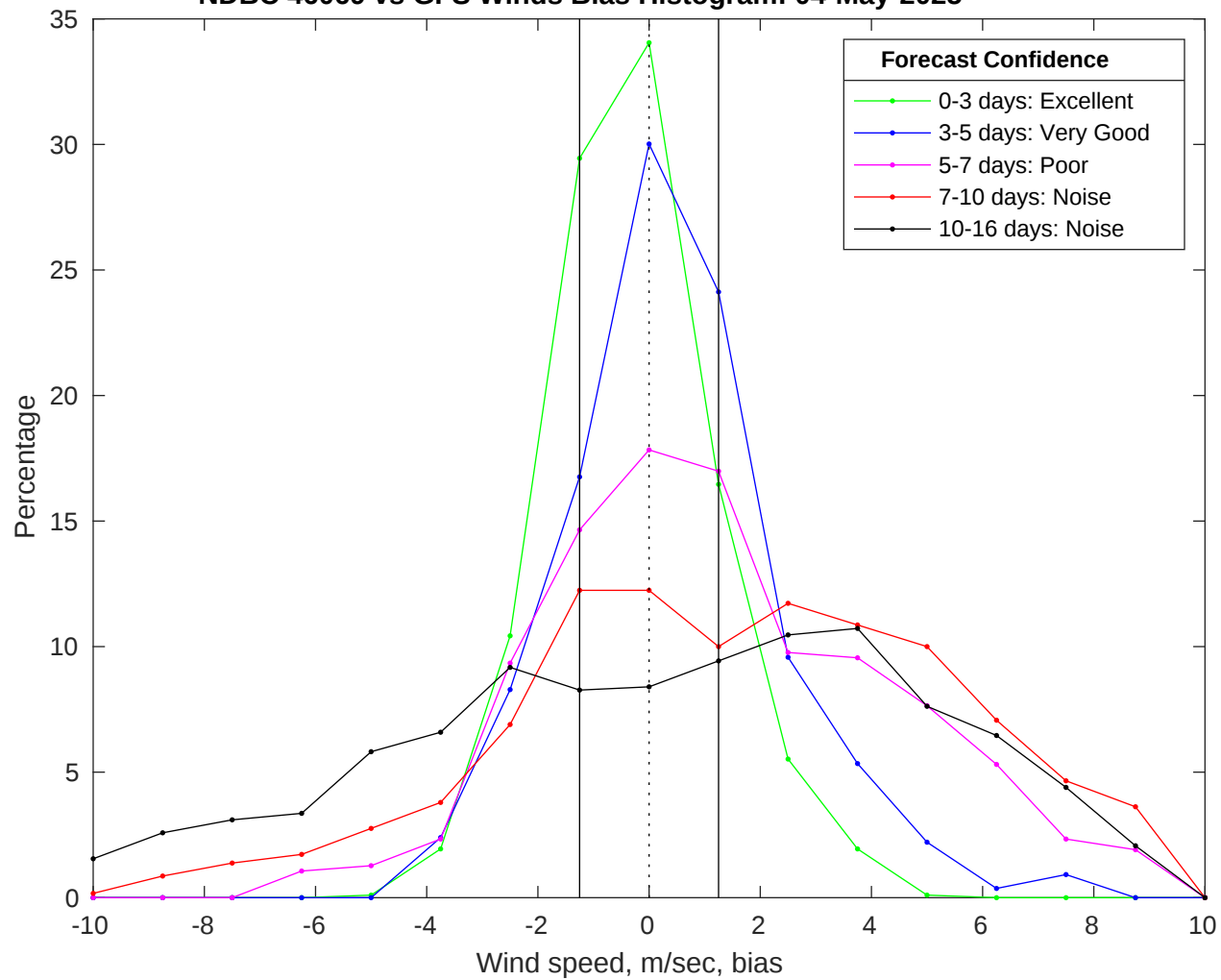
NDBC 46069 vs GFS Winds Bias Histogram: 04-May-2025
