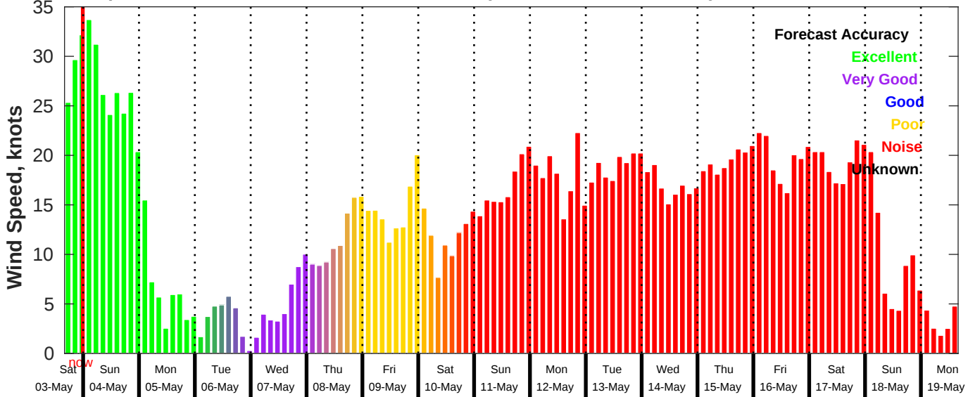
GFS Wind Speed Forecast for NDBC 46069 from 03-May-2025 16:00:00 to 19-May-2025 16:00:00
