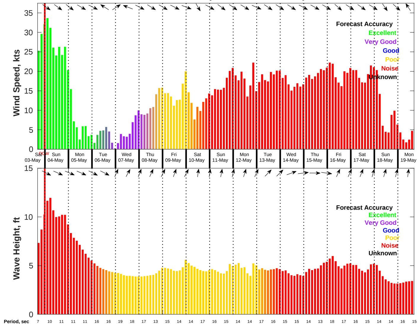
Wind & Wave Forecast for NDBC 46069 from 03-May-2025 16:00:00 to 19-May-2025 16:00:00
