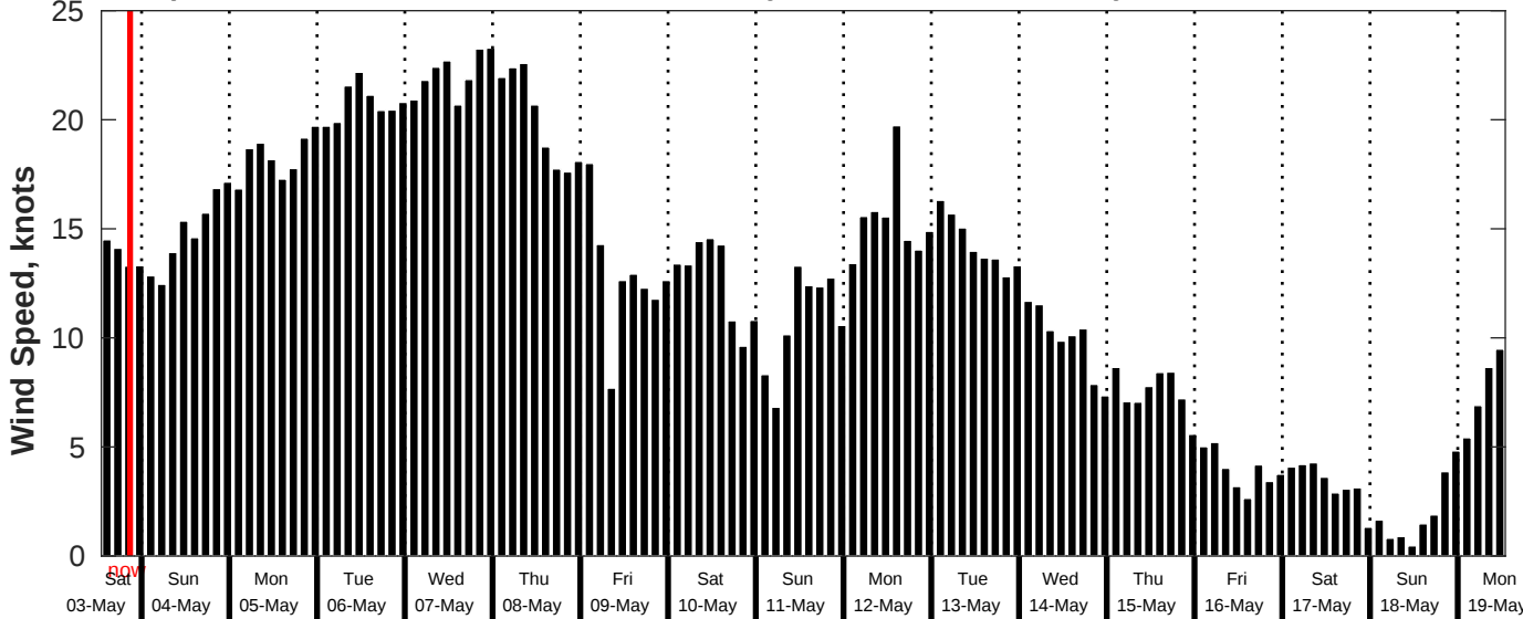
GFS Wind Speed Forecast for NDBC 51209 from 03-May-2025 13:00:00 to 19-May-2025 13:00:00
