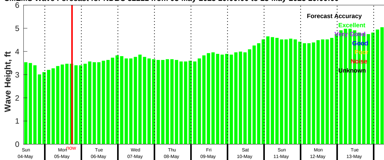
CMEMS Wave Forecast for NDBC 52211 from 03-May-2025 10:00:00 to 13-May-2025 10:00:00
